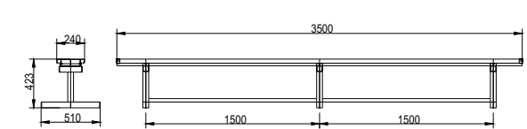
LP-1 LP-1 One-Row Bleacher Without Back Bleacher Size 3500(W)X510(D)X423(H)mm Seat Board Size 3500(W)X240(D)X60(H)mm
