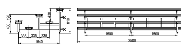
LP-3 LP-3 Three-Row Bleacher Without Back Bleacher Size 3500(W)X1540(D)X810(H)mm Seat Board Size 3500(W)X240(D)X60(H)mm Step Size 3500(W)X240(D)X60(H)mm
