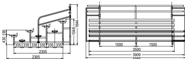
LD-4 LD-4 Four-Row Bleacher With Low Back Bleacher Size 4086(W)X2305(D)X1644(H)mm Seat Board Size 3500(W)X333(D)X110(H)mm Step Size 3909(W)X240(D)X60(H)mm
