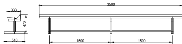
LD-1 LD-1 One-Row Bleacher With Low Back Bleacher Size 3500(W)X510(D)X470(H)mm Seat Board Size 3500(W)X333(D)X110(H)mm
