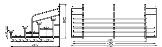
LP-4 LP-4 Four-Row Bleacher Without Back Bleacher Size 4086(W)X2305(D)X1602(H)mm Seat Board Size 3500(W)X240(D)X60(H)mm Step Size 4000(W)X240(D)X60(H)mm
