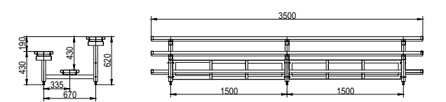
LP-2 LP-2 Two-Row Bleacher Without Back Bleacher Size 3500(W)X670(D)X620(H)mm Seat Board Size 3500(W)X240(D)X60(H)mm Step Size 3500(W)X240(D)X60(H)mm
