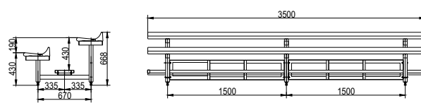
LD-2 LD-2 Two-Row Bleacher With Low Back Bleacher Size 3500(W)X670(D)X668(H)mm Seat Board Size 3500(W)X333(D)X110(H)mm Step Size 3500(W)X240(D)X60(H)mm
