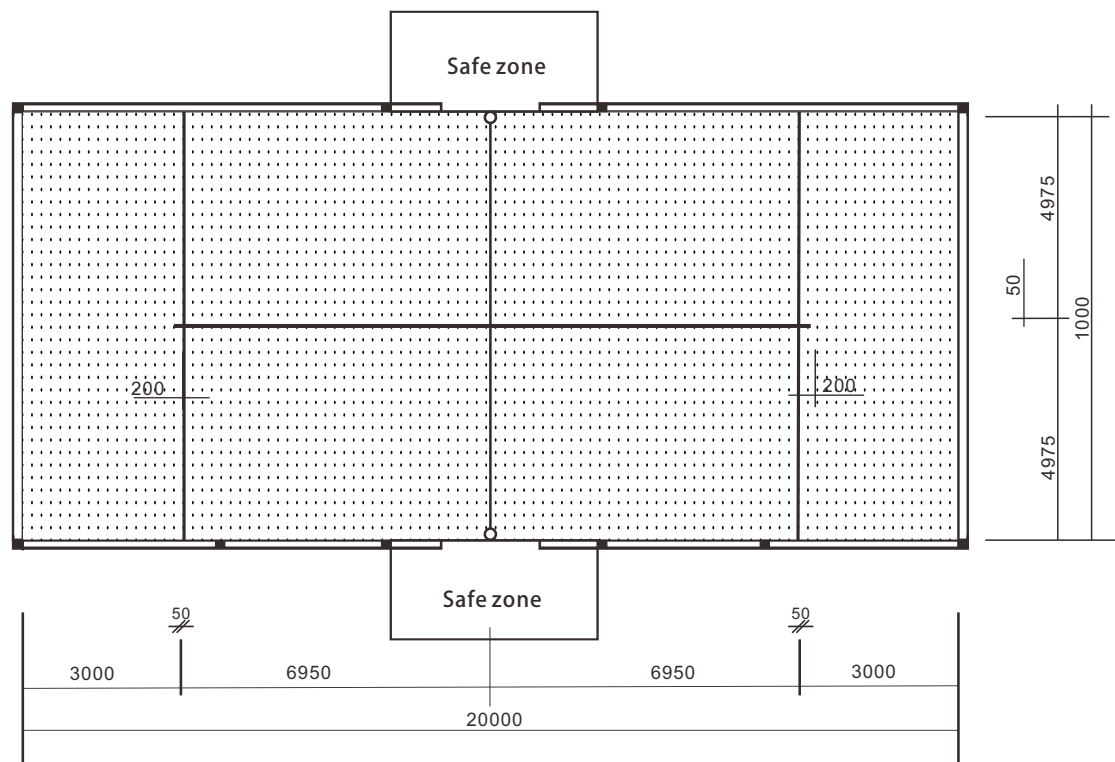
Doubles padel court length 20meter,width 10m,diagonal 22.36m
