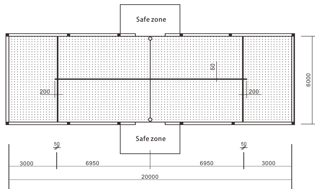
Singles padel court length 20meter,width 6m,diagonal 20.88m
